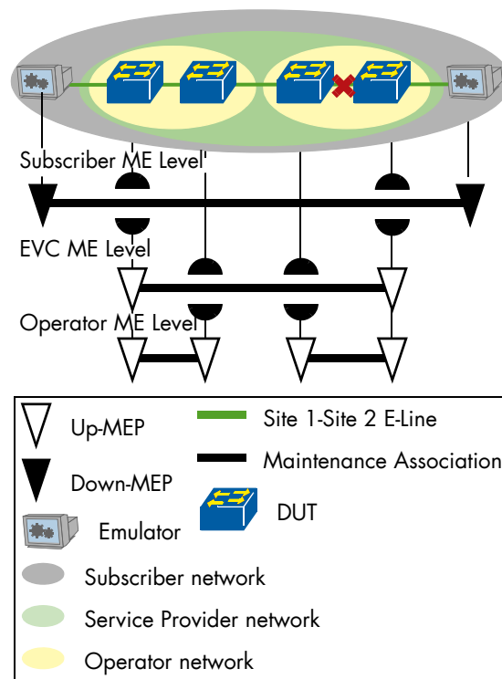
Figure 3: Hierarchical Service OAM
